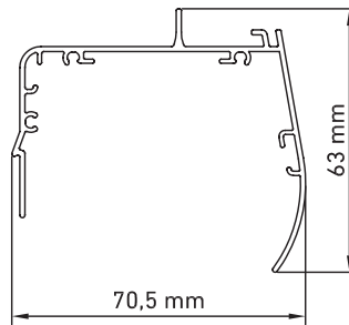
Semi cajón 70 Half box 70 Demi caisson 70
