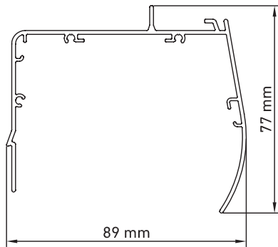
Semi cajón 90 Half box 90 Demi caisson 90
